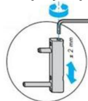
Regulating the height
