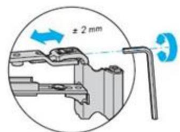
Regulating the frame position
